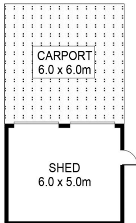
CARPORT/SHED (NOT TO SCALE)
