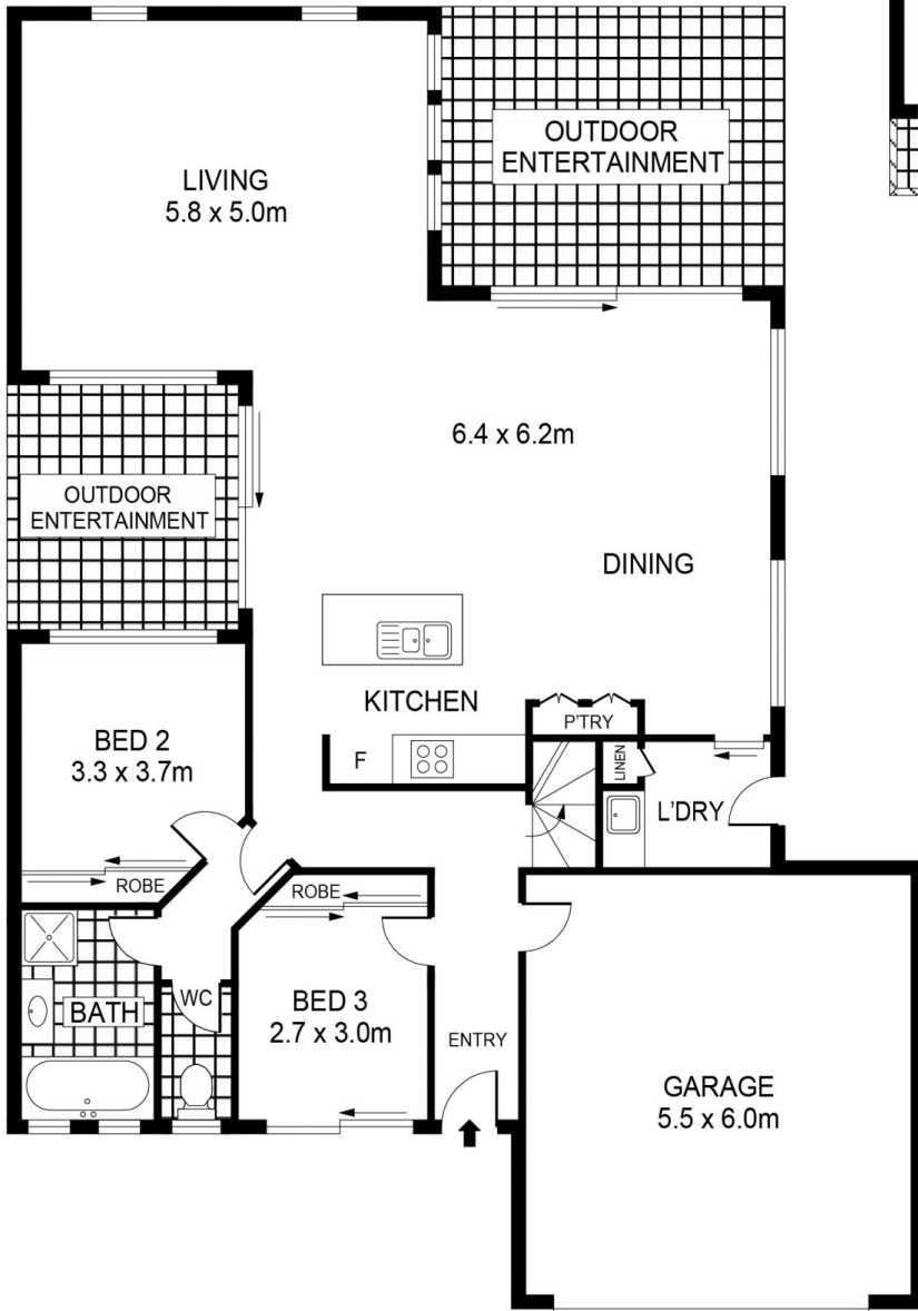
GROUND FLOOR
